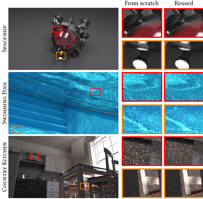
Fig. 13. Learned distributions can be reused for novel camera views. The right column shows results where the network weights were initialized with weights learned for camera views in Figure 8.
