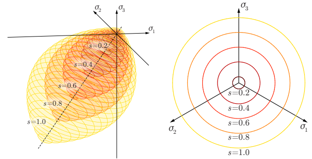
Fig. 4. Failure Potential. Bresler-Pister failure surfaces for several scale factor values s (left). Intersection curves with the deviatoric plane (right) motivate the use of s as a measure of distance to failure.
