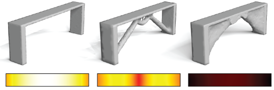
Fig. 14. Failure Objective Energy Landscape We show the energy landscape (bottom) of the objective f_{\text{fail}} for all positions of a load applied to the top surface of the bridge. For an unoptimized bridge (left), the load location that leads to the highest energy—the location of the worst-case load—is in the center. For the fixed-load optimized bridge (center), the locations for the worst-case loads move to the two ends, and the effect of these loads is weaker. The bridge optimized under worst-case loads (right) no longer has any load locations that would lead to failure.
