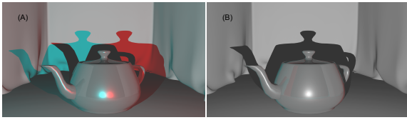
Figure 3: Left: rendering S3D with shifted lights. Right: shading stereo is applied to the teapot only.
