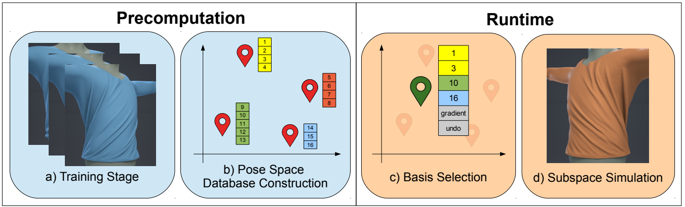
Figure 2: Overview of our pipeline: (a) We perform full-space cloth simulation to create training data — shown in blue. (b) We construct a Pose Space Database — a simplified 2D view with four sites and 16 basis vectors in total is illustrated. (c) At runtime, we adaptively select vectors from the database to obtain a basis for the current pose — in this case two from the yellow site, one from the green one, one from the blue one, plus gradient and undo vector. (d) We solve the subspace simulation problem using the selected basis — shown in orange.
