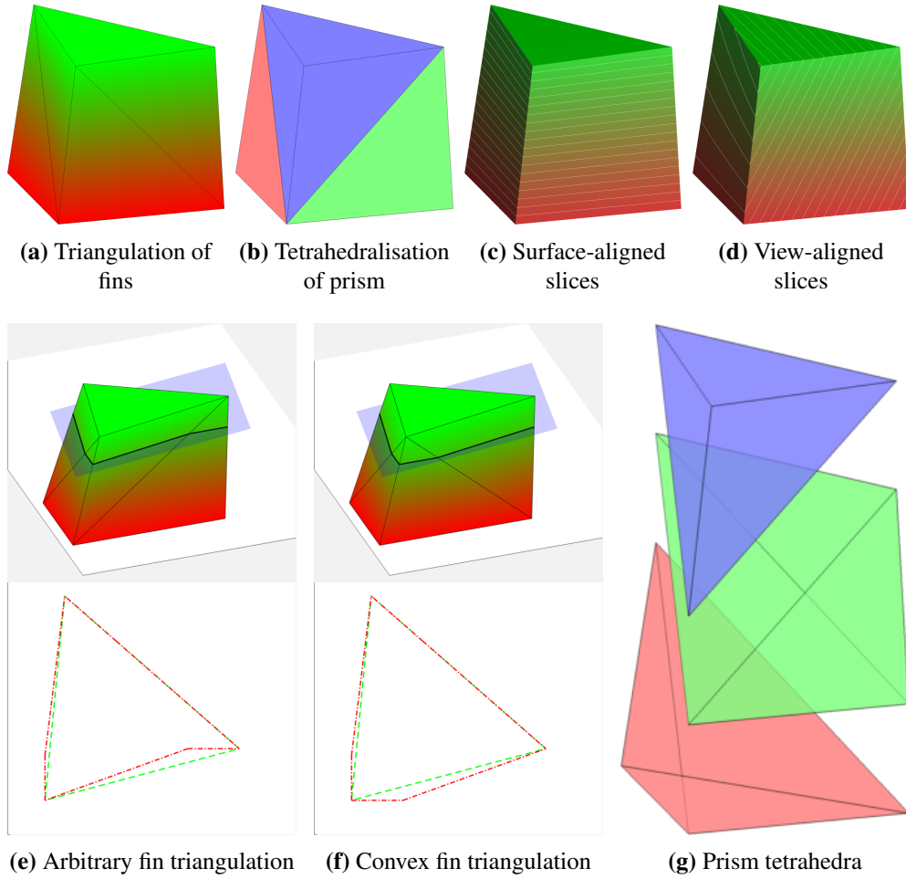
Figure 7. Shell geometry representations for rendering. Bottom parts of subfigures 7e and 7f show the horizontal slice of the prism from a top view using green colour for the original prism volume silhouette and red for the fin approximation with triangles.
