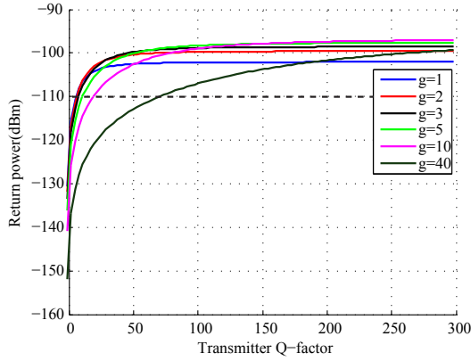
Fig. 6. The calculated return power vs. transmitter Q-factor for various over-coupling ratios ( g ), for Q_{rx} = 20 , and k = 0.01 . It shows that increasing the Q-factor increases the load modulation power that reaches the reader. The dashed line shows a typical value for the sensitivity of the reader chip.
