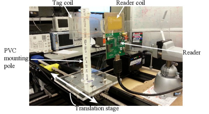
Fig. 10. Photograph of the experimental setup for measuring the read range. The RFID reader is TRF7070 A development kit.
