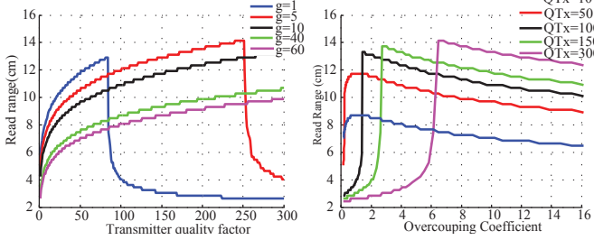
Fig. 9. (a) Shows the impact of increasing Q-factor for given values of g (b) Shows the value of g_{min} for certain values of Q-factor of transmitter.
