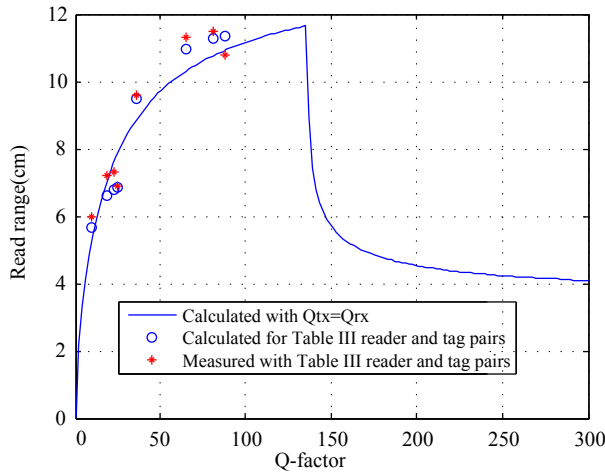
Fig. 13. Maximum reading distance versus quality factor. For Q_{tx} \neq Q_{rx} , Q is defined as the geometric mean of Q_{rx} and Q_{tx} . Measurement is the actual reading range using TRF7970A development kit.
