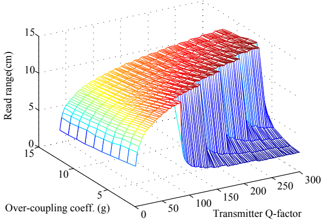
Fig. 8. The maximum reading distance vs. Q-factor of transmitter for varied over-coupling coefficients ( g ).
