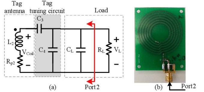
Fig. 12. (a) Shows the circuit diagram of the receiver side b) shows the receiver antenna and tuning circuit (Chip is soldered to an SMA connector to be attached to antenna)
