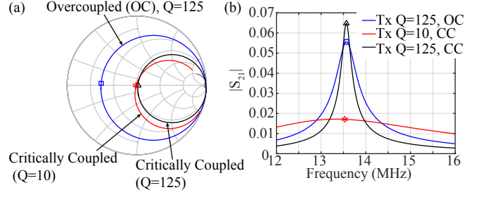
Fig. 2. (a) Smith chart illustrating impedance variation over frequency for OC and CC resonators, with high and low Q values. (b) Magnitude of the transmission coefficient, |S_{21}| corresponding to the impedances plotted in panel (a). In this example, the coupling coefficient, k = 0.005 . The blue square, red asterisk (*), and black triangle indicate the frequency at which f = 13.56 MHz on each curve for the Q = 125 OC, Q = 10 CC, and Q = 125 CC cases, respectively.
