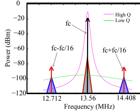
Fig. 5. A typical spectrum of an HF RFID system illustrating the reader command and the load modulation. The impact of increasing the reader Q-factor on the bandwidth and the load modulation is shown.
