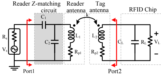
Fig. 1. Circuit schematic showing tuning circuit for reader and tag antennas and also the RFID chip lumped model
