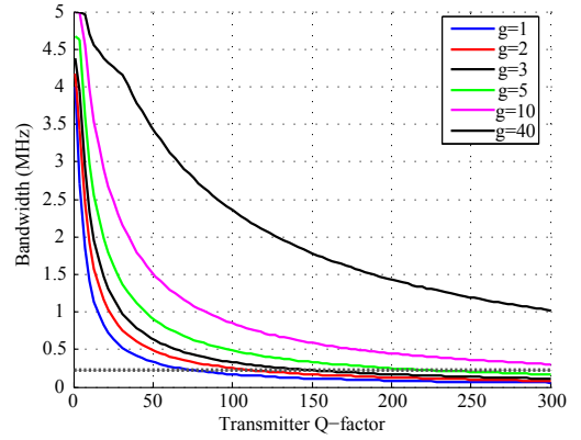
Fig. 7. The calculated bandwidth vs. reader Q-factor for various over-coupling coefficients ( g ) for Q_{rx} = 20 , and k = 0.01 . The grey dotted-line shows the minimum bandwidth required for a 14443 type A with 106 kb/s bit rate discussed earlier as an example. Over-coupled tuning increases the bandwidth and enables use of higher Q reader antennas.
