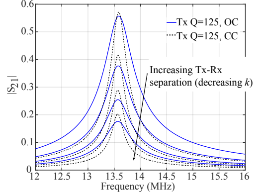
Fig. 4. |S_{21}| , between the transmitter and load (RFID chip), for varied separations between transmitter and receiver from 3.8 to 6.8 cm. Note that, due to overcoupling, the resonance of the OC case is damped compared to the CC case, yielding a desirably larger bandwidth.
