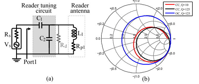
Fig. 11. (a) Circuit diagram of the antenna and tuning circuit (b) The Smith chart shows the measured S_{11} for 3 design cases considered in this work: CC, Q=10 ; CC, Q=125 ; and OC, Q=125 .
