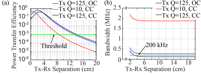
Fig. 3. (a) Power transfer efficiency for the circuit of Fig. 1 as the distance between transmitter and receiver is varied for an OC transmitter with Q = 125 , a CC transmitter with Q=10 , and a CC transmitter with Q=125 . (b) Bandwidth versus reader to tag coil separation for same Q and OC/CC combinations of panel (a).
